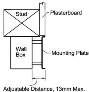
Figure 1. Adjustment Distance as Viewed from Above
