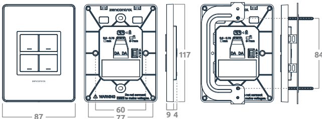
zc-sceneset-c-a4 Dimensions 87 / 117 / 13 mm Mounting centres 80 mm
