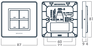
zc-sceneset-a4 Dimensions 87 / 87 / 13 mm Mounting centres 64 mm
